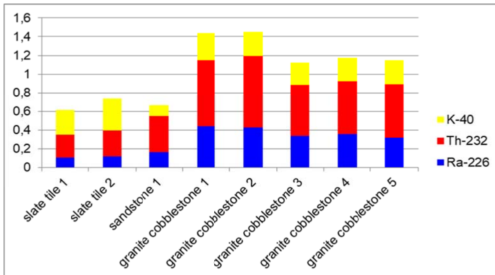
Figure 9.7 : relative contribution of K-40, Th-232 and Ra-226 to the index I for slate and sandstone tiles and for granite cobble stones.
