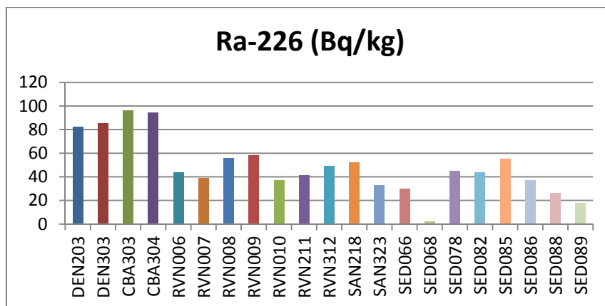
Fig. 8.2: activity concentration of radium-226 in sediments of Walloon watercourses.
