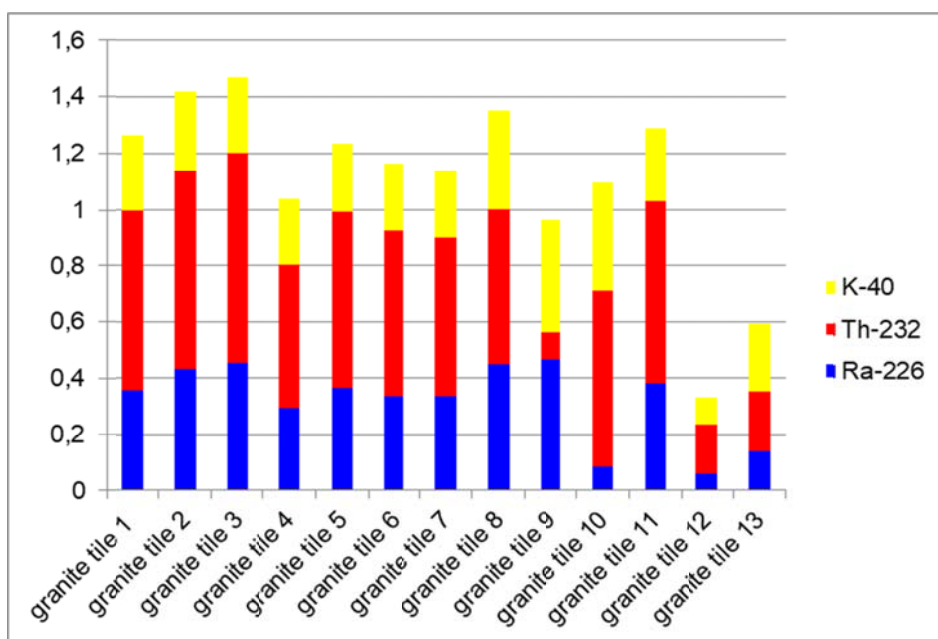
Figure 9.6 : relative contribution of K-40, Th-232 and Ra-226 to the index I for granite tiles
