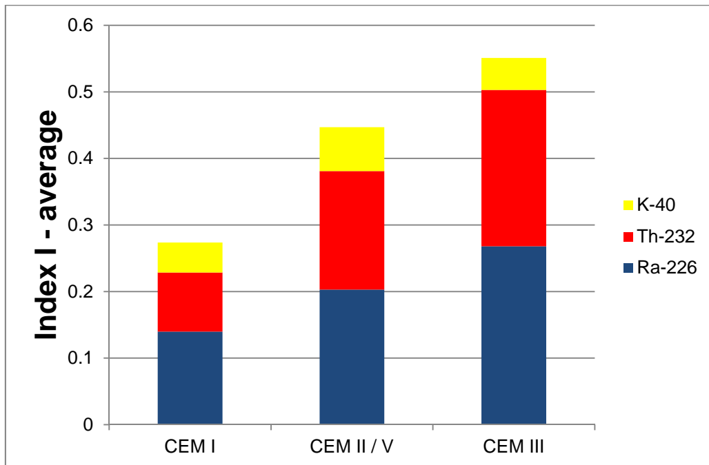
Figure 9.1 : relative contribution of K-40, Th-232 and Ra-226 to the index I for cement.
