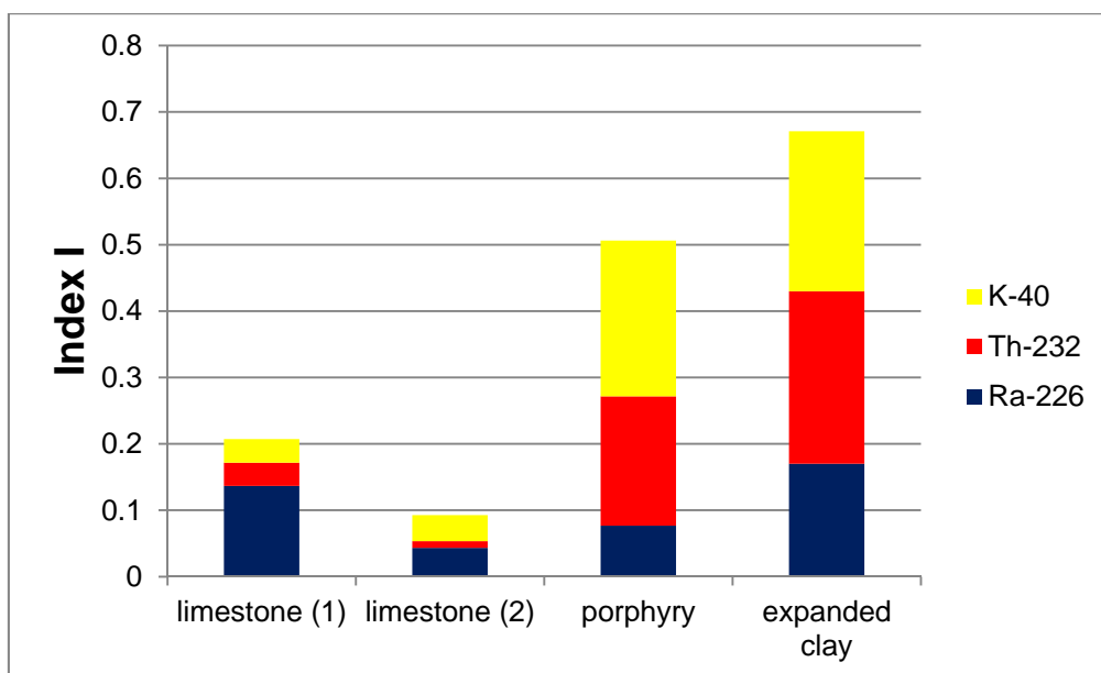
Figure 9.3 : relative contribution of K-40, Th-232 and Ra-226 to the index I for aggregates
