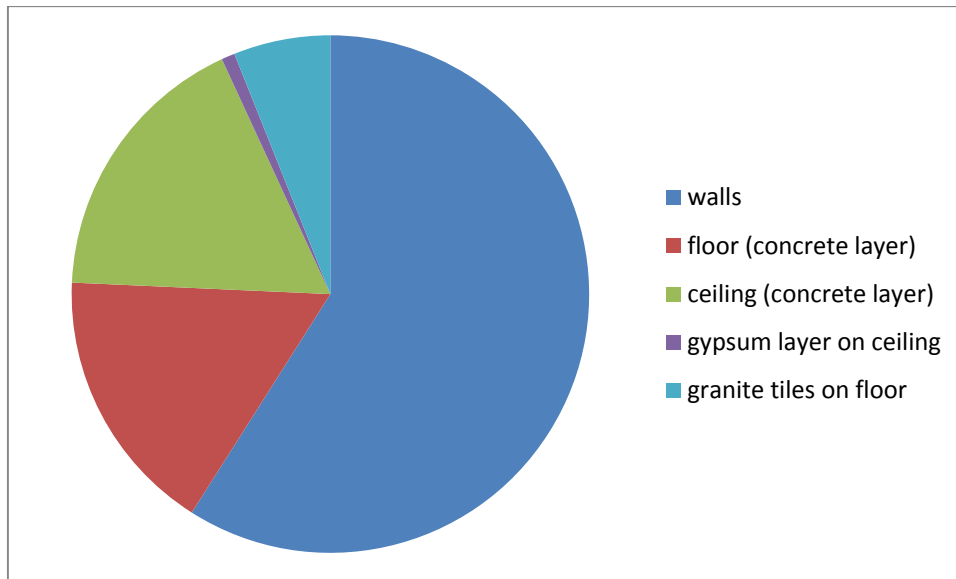
Fig. 9.9 : respective contributions of each element of the « standard room » to the external dose
