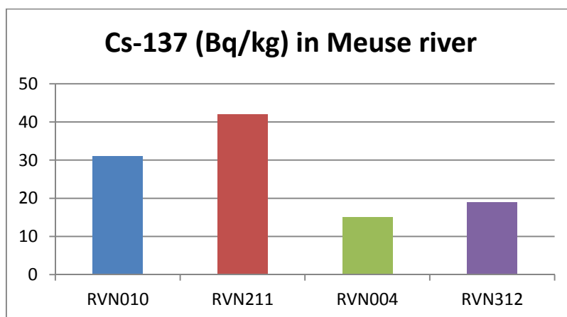
Fig. 8.1 : Cs-137 activity concentration in the Meuse river; sampling points from stream upwards to downwards (RVN010 – Dinant, RVN211- Namur, RVN004 – Huy, RVN312 – Visé).
