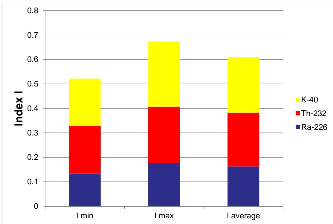
Figure 9.4 : relative contribution of K-40, Th-232 and Ra-226 to the index I for bricks
