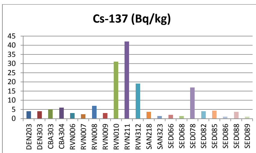
Fig. 8.3: activity concentration of cesium-137 in sediments of Walloon watercourses.
