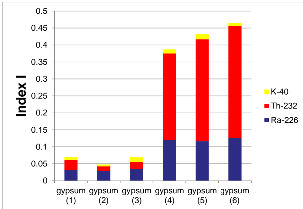
Figure 9.5 : relative contribution of K-40, Th-232 and Ra-226 to the index I for gypsum
