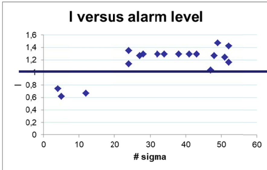
Figure 9.8 : activity index of natural stones as a function of alarm level on the portal monitor.
